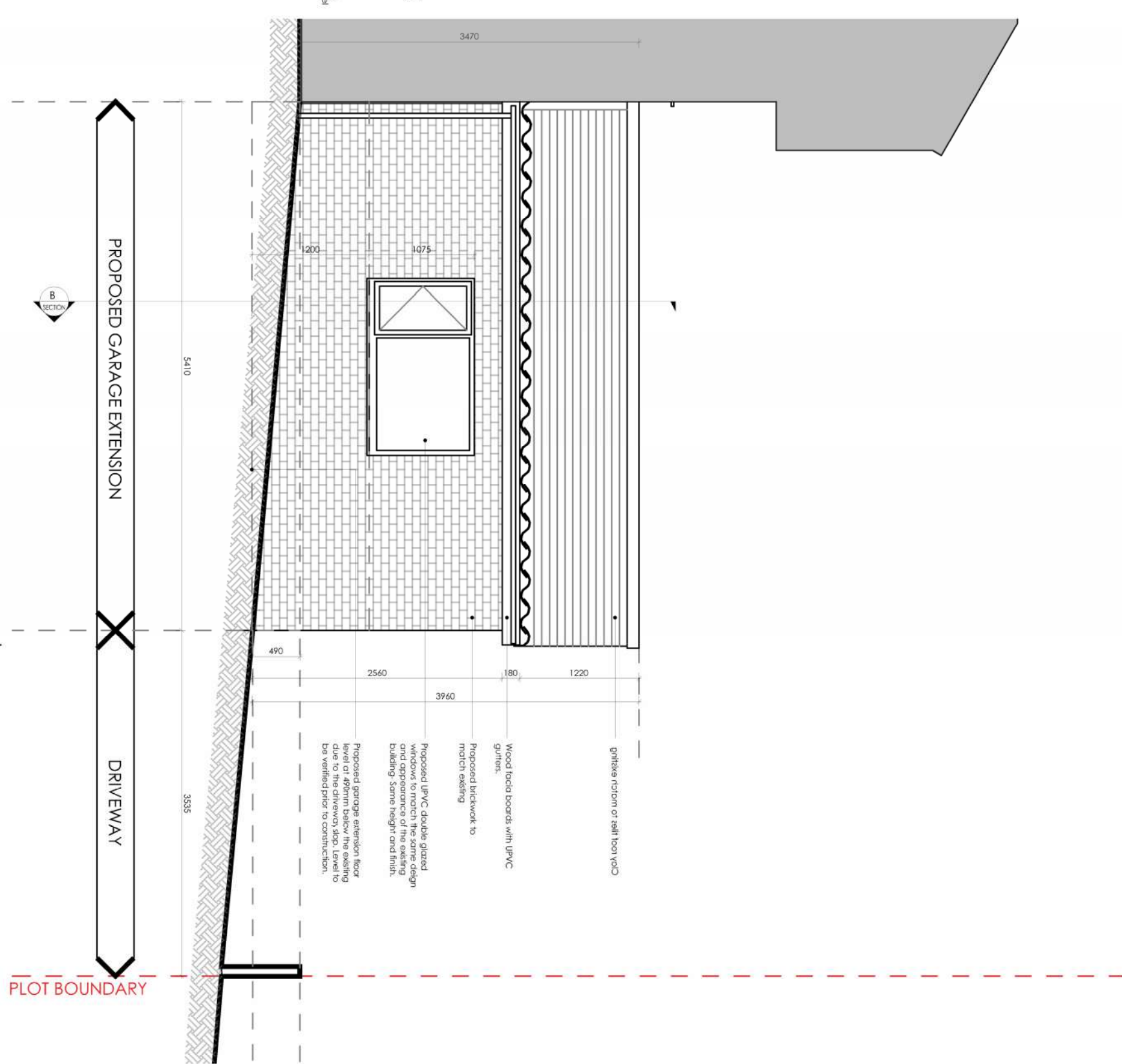
2. PROPOSED ELEVATION_S/E FACING
