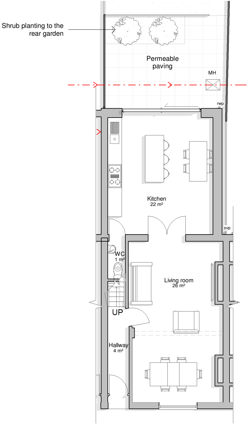
Ground Floor 1 : 100
