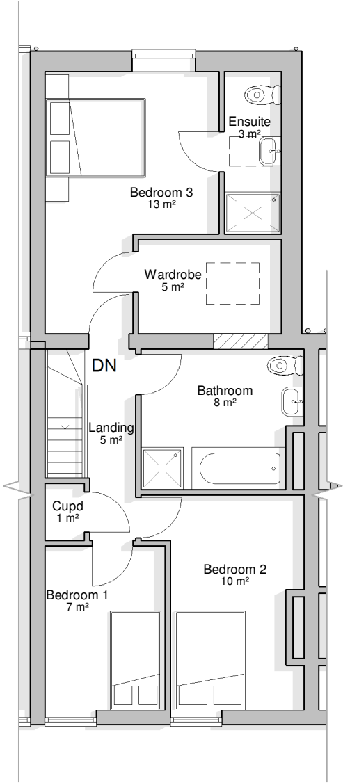
First Floor 1 : 100
