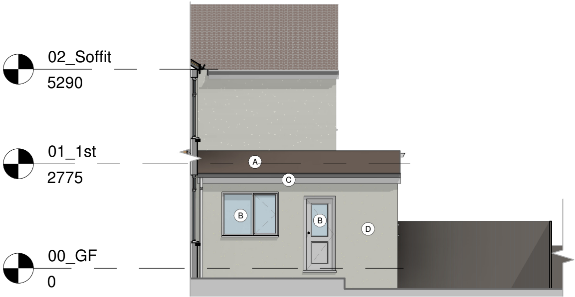
South East (Side) Elevation 1 : 100
