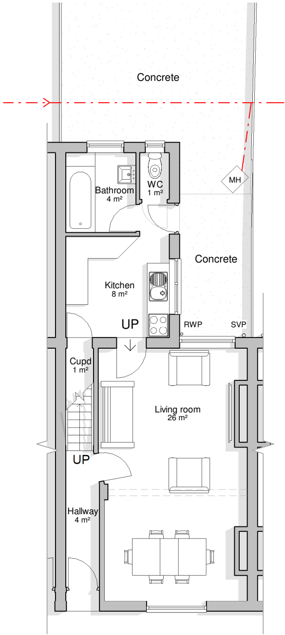
Ground Floor 1 : 100
