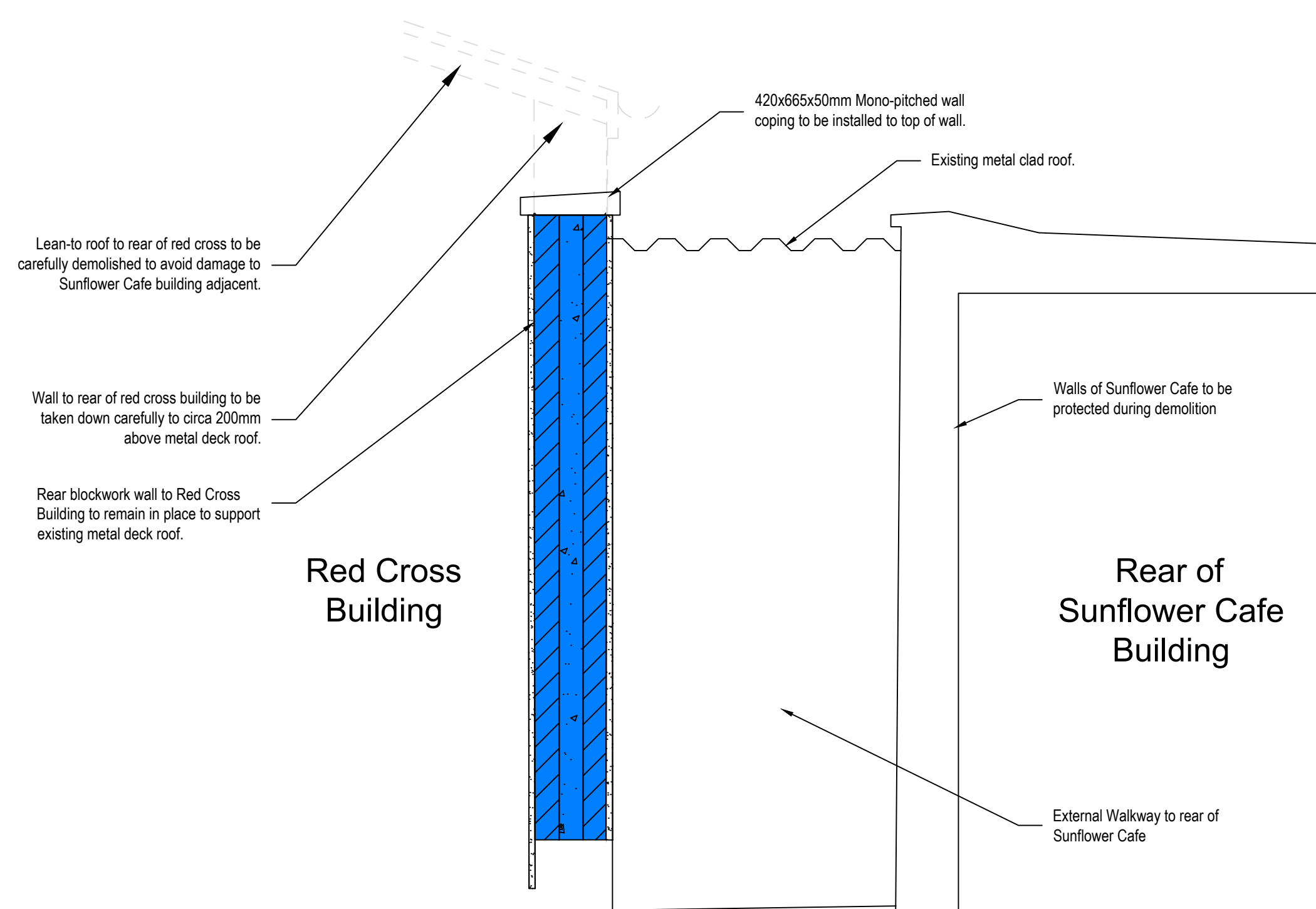
Section 1 Showing Proposed Remedial Works at Red Cross Boundary Wall
