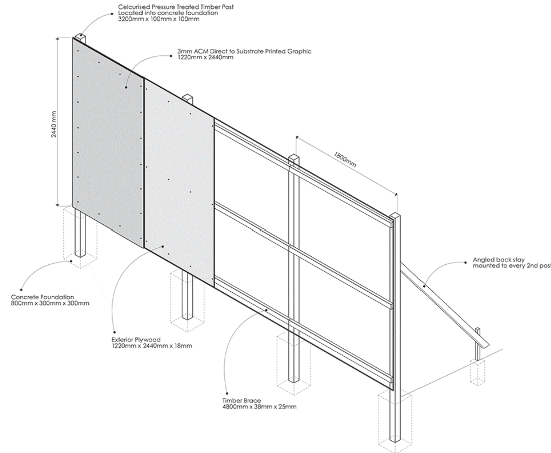
2.44m High Timber Hoarding Detail NTS
