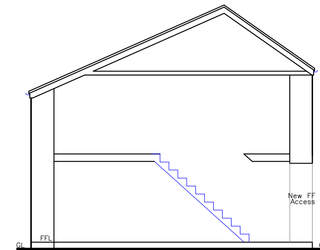
Proposed Section 1:100
