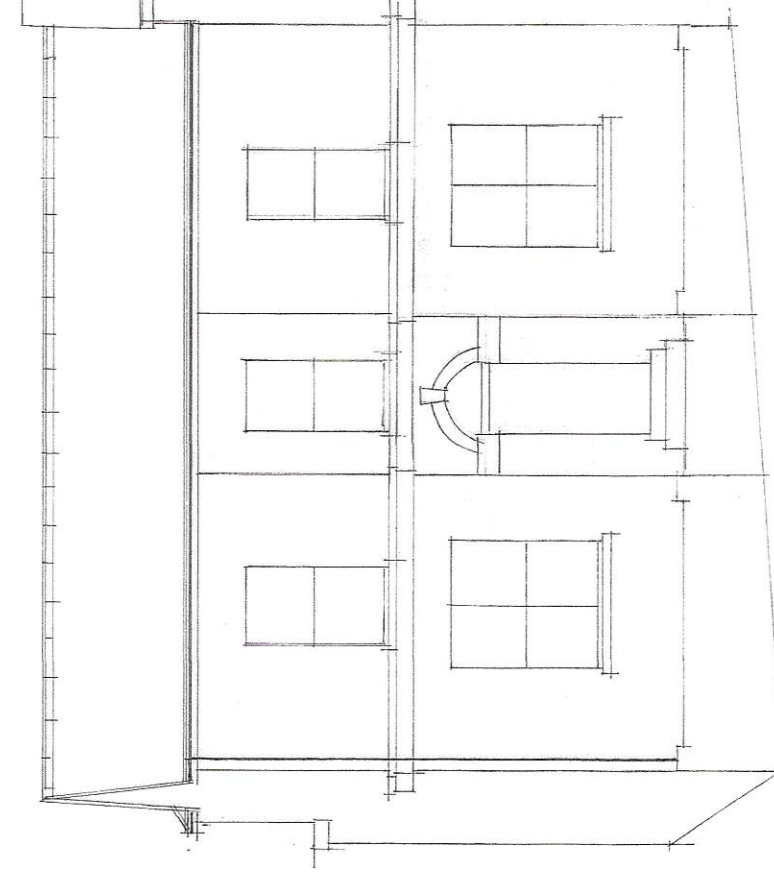
Proposed Front Elevation - south
