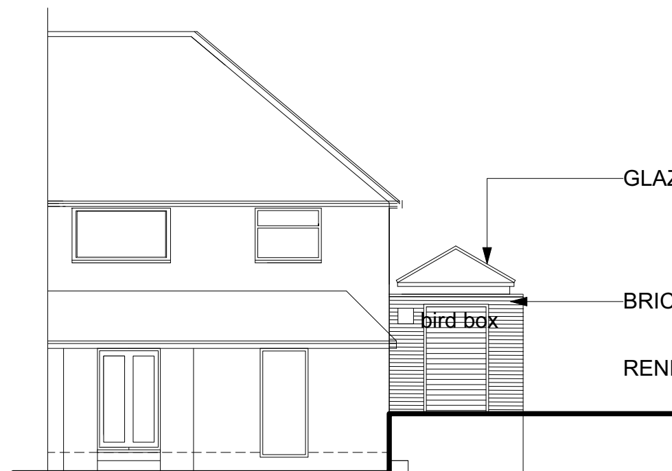
FRONT ELEVATION
