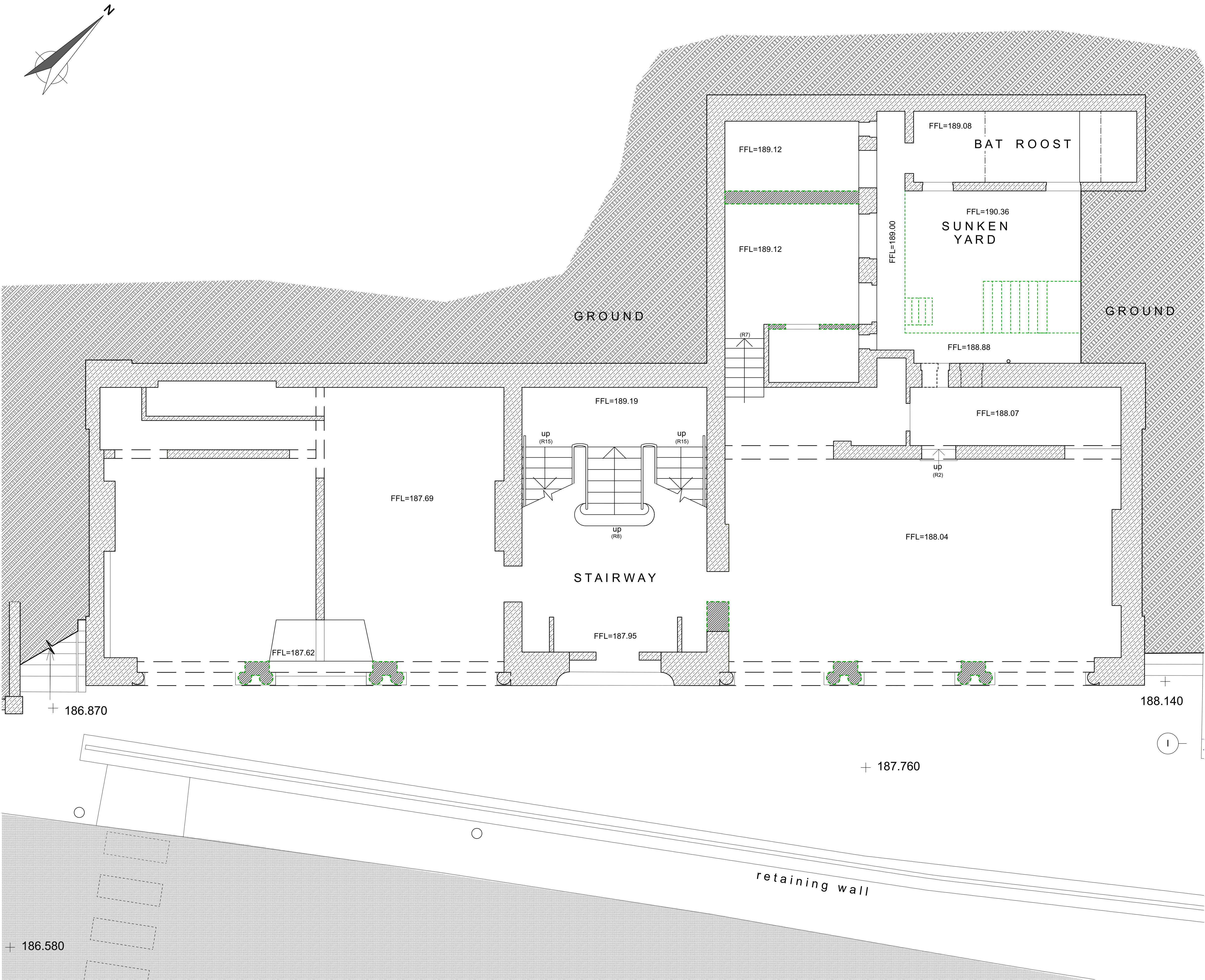
1 Ground Floor Demolition Plan Scale: 1:50
