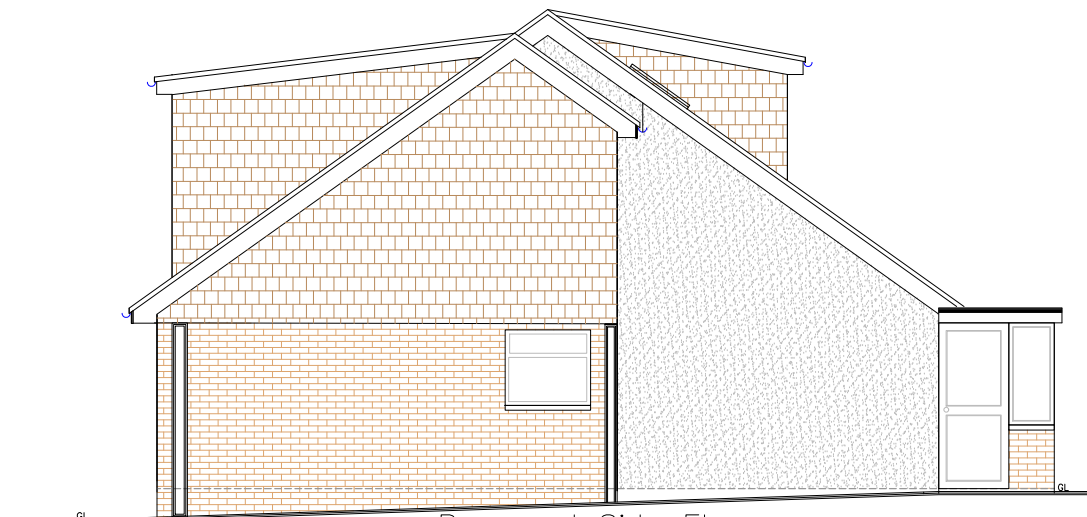
Proposed Side Elev 1:100
