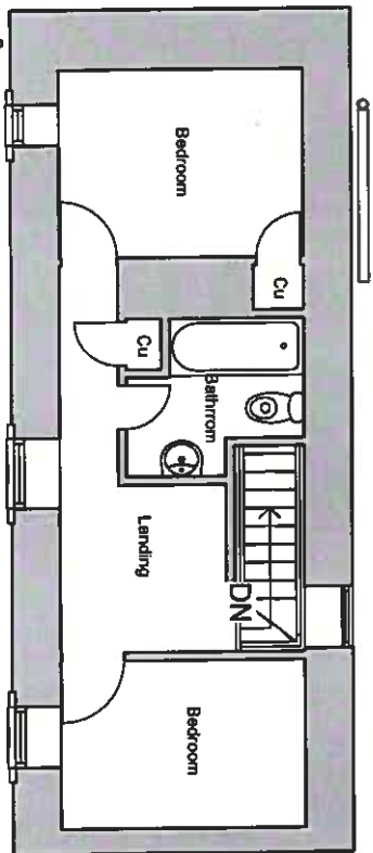
2 Proposed First Floor 1 : 100
