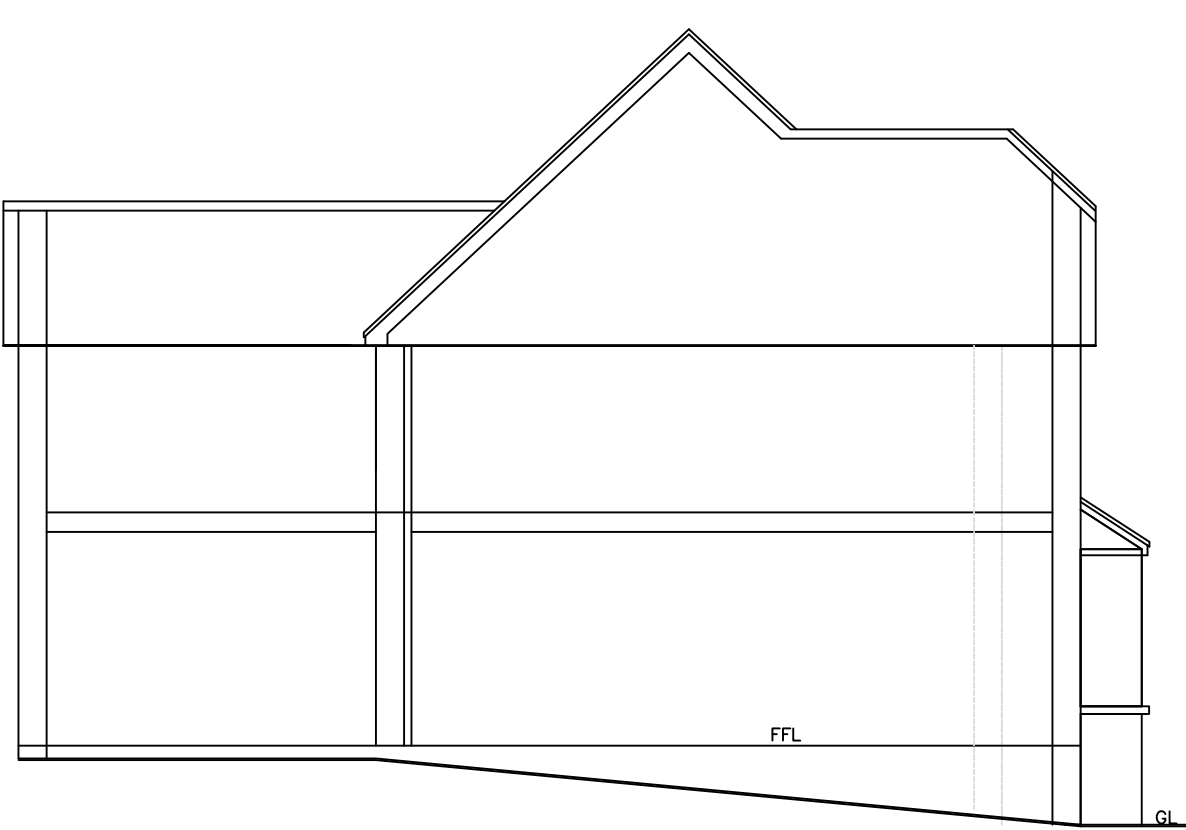
Existing Section 1:100
