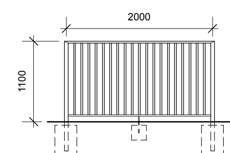
RAILINGS TO MATCH EXISTING 1:50
