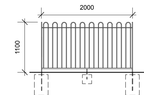
HOOP TOP RAILINGS 1:50
