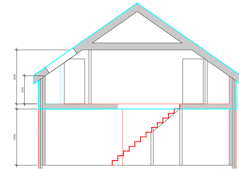
Attic First Floor Section
