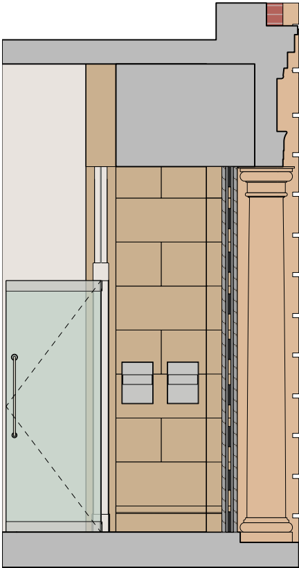
A 560.4 ELEVATION C SCALE 1:25 @ A1, 1:50 @ A3
