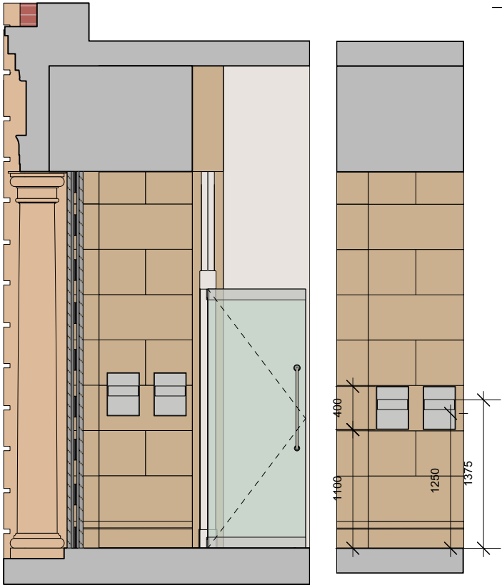
A 560.2 ELEVATION A SCALE 1:25 @ A1, 1:50 @ A3
