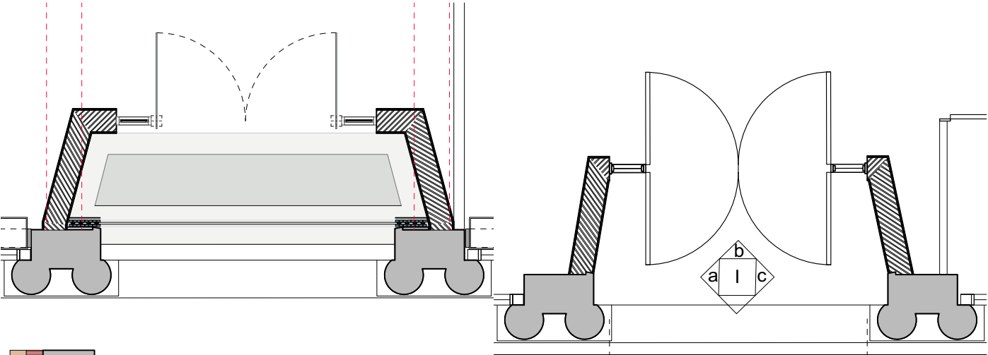
A 560.1 EXTERIOR ELEVATION SCALE 1:100 @ A1, 1:50@ A3
