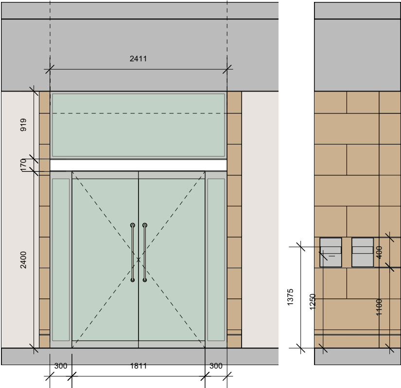
A 560.3 ELEVATION B SCALE 1:25 @ A1, 1:50 @ A3
