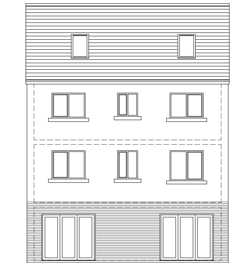
WEST ELEVATION
