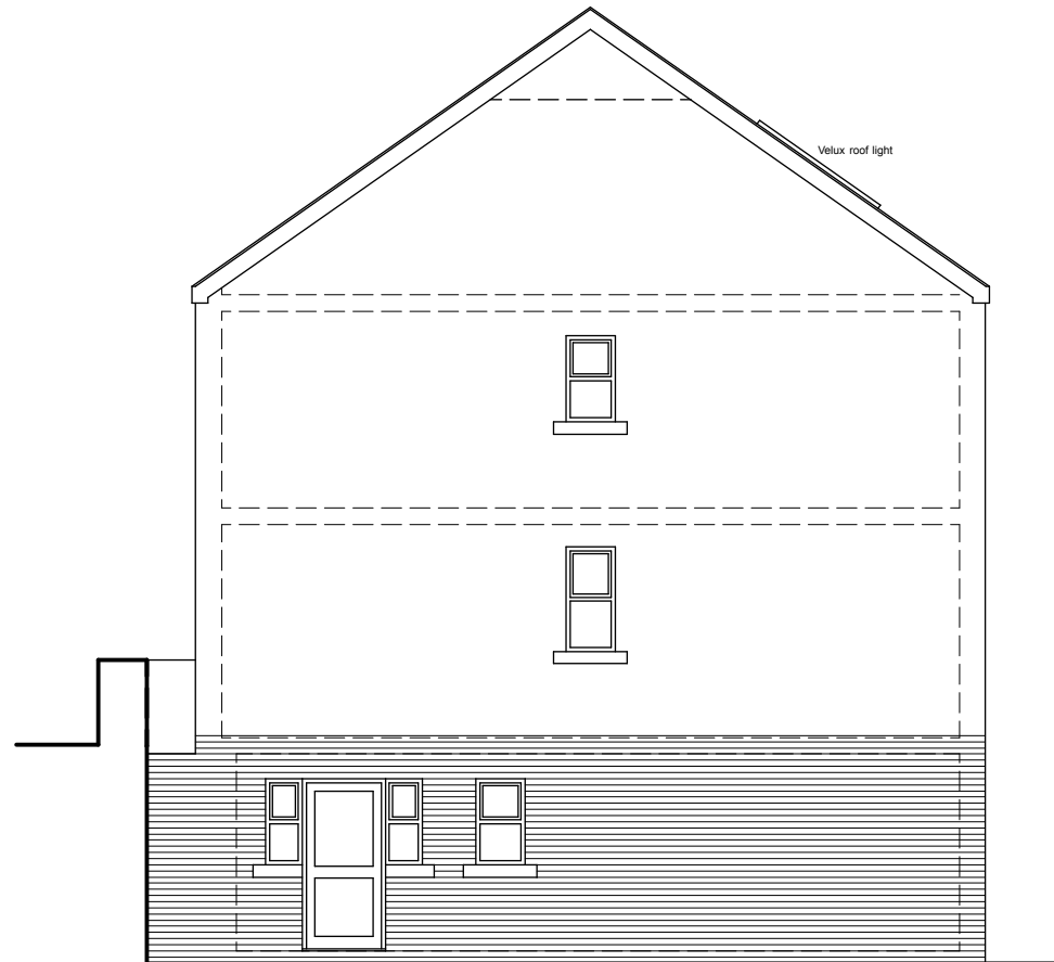
NORTH ELEVATION
