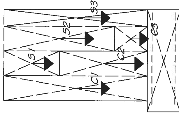
FORCE DIAGRAM 1:20
