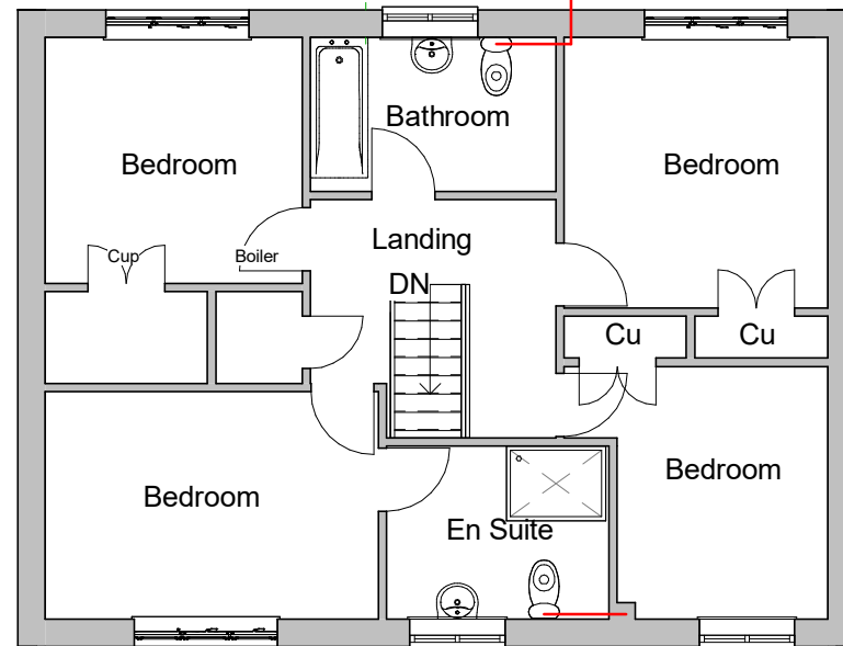
2 First Floor 1 : 100
