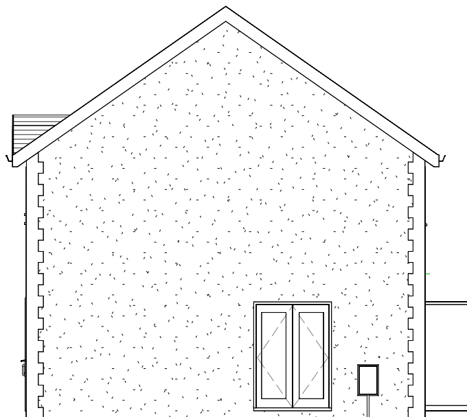
6 Side 2 Elevation 1 : 100
