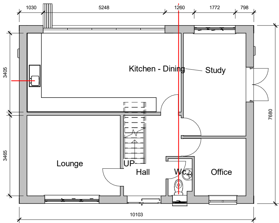
1 Ground Floor 1 : 100
