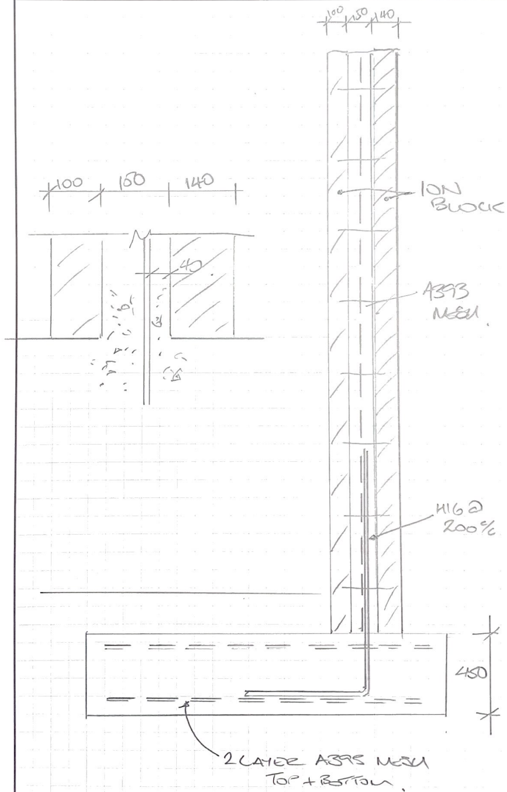
TYPICAL SECTION THROUGH RETAINING WALLS TO HOUSES
