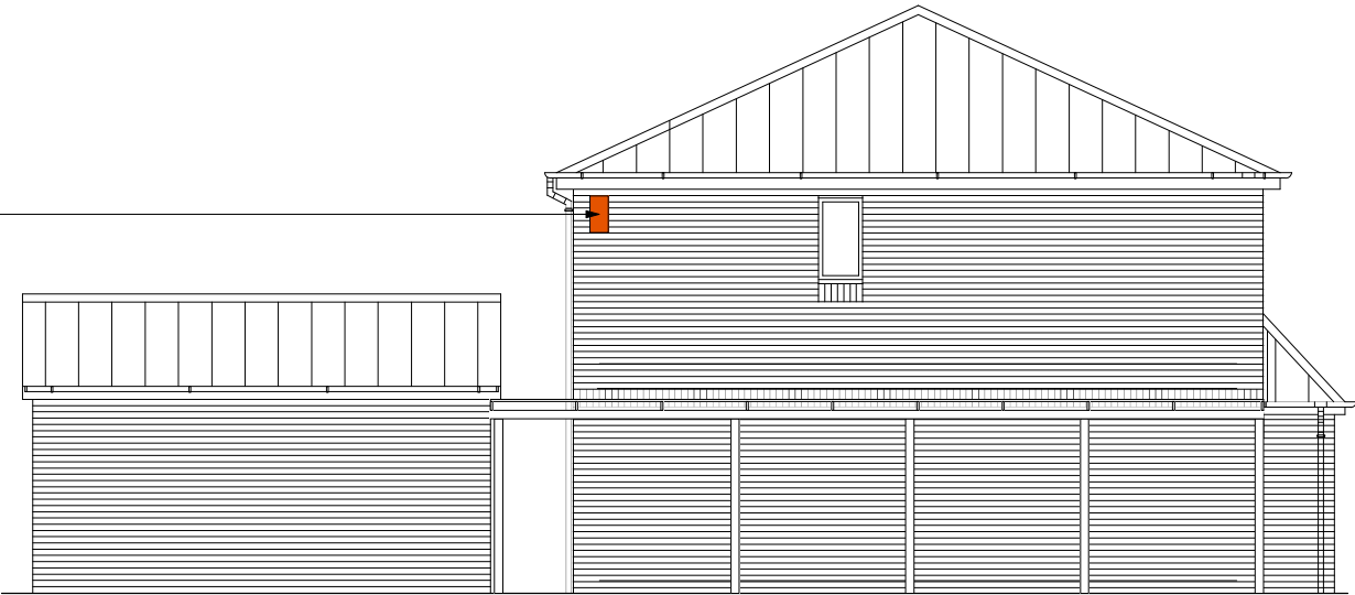
Proposed Elevations Side
