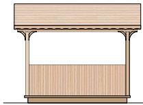
Proposed Side Elevation
