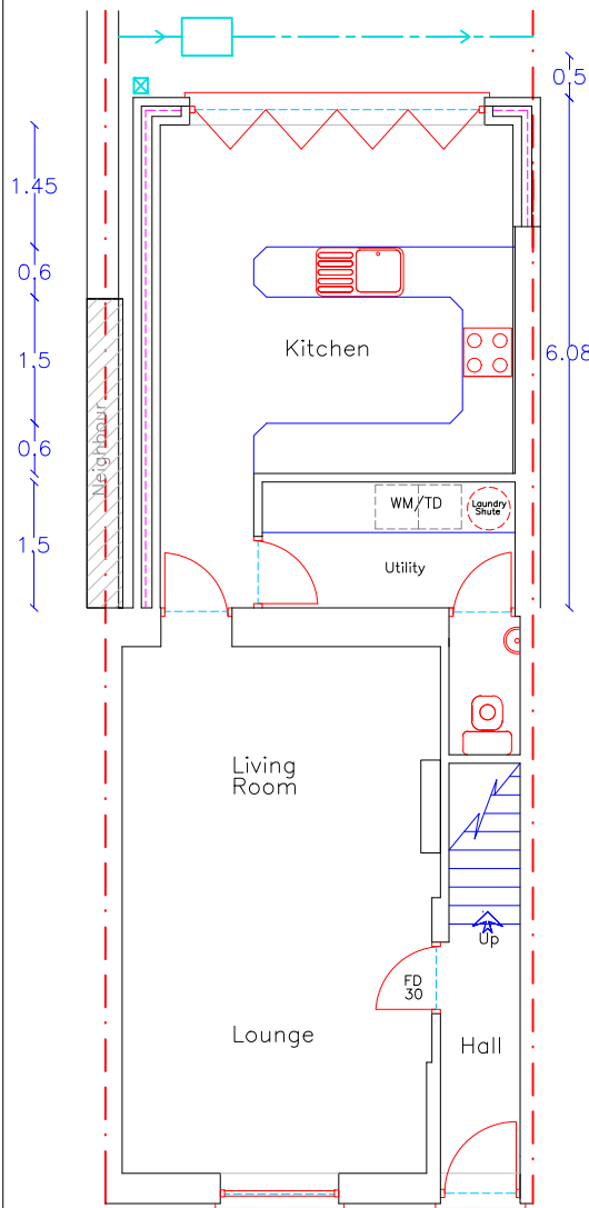
Proposed Ground Floor Plan 1:100
