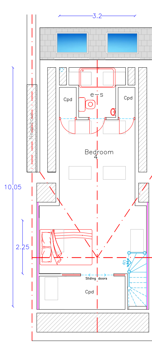
Proposed Loft Floor Plan 1:100
