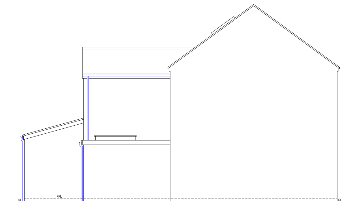
Existing Side Elev 1:100
