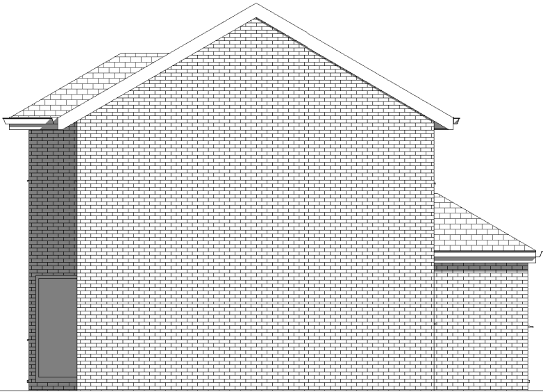
3 Proposed Side 1 Elevation 1 : 100
