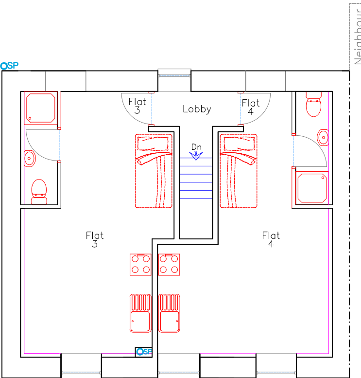
Proposed F Floor Plan 1:100
