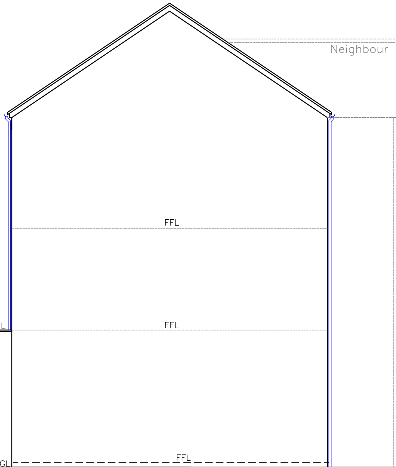
Proposed Side Elevation 1:100
