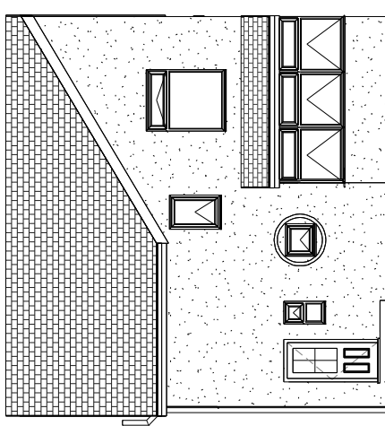
① Existing Front Elevation 1 : 100
