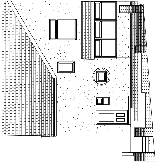
⑤ Existing Front Garden Elevation 1 : 100
