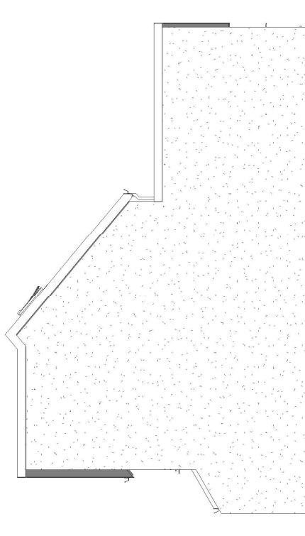
④ Existing Side 2 Elevation 1 : 100
