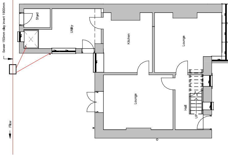
① Existing Ground Floor 1 : 100
