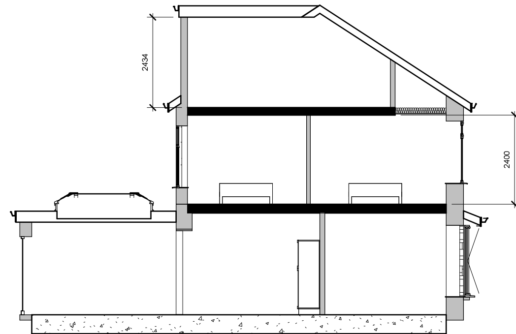
2 Proposed Section 1 : 100
