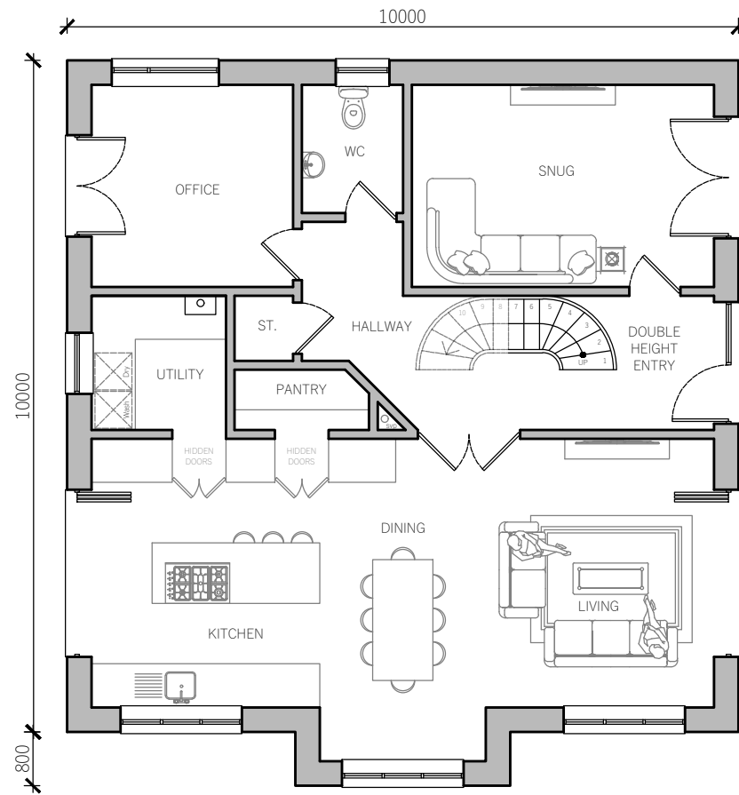
GROUND FLOOR PLAN 1:00
