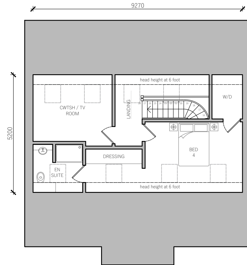
LOFT FLOOR PLAN 1:00
