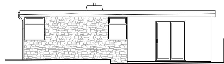
NORTH ELEVATION 1:00
