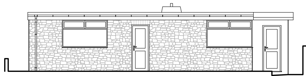
EAST ELEVATION 1:00
