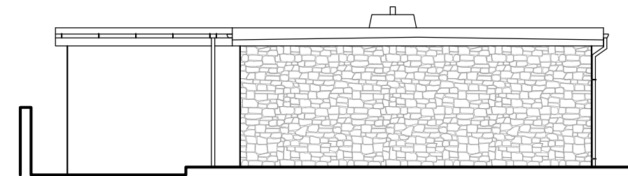
SOUTH ELEVATION 1:00
