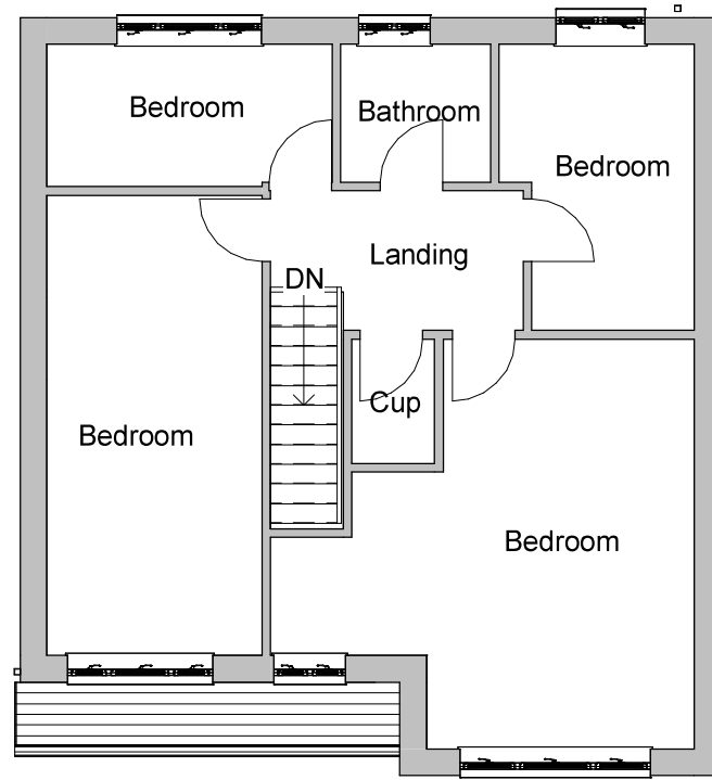
2 Existing First Floor 1 : 100
