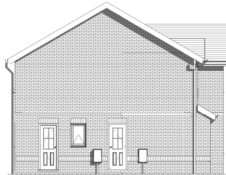
5 Existing Side 1 Elevation 1 : 100
