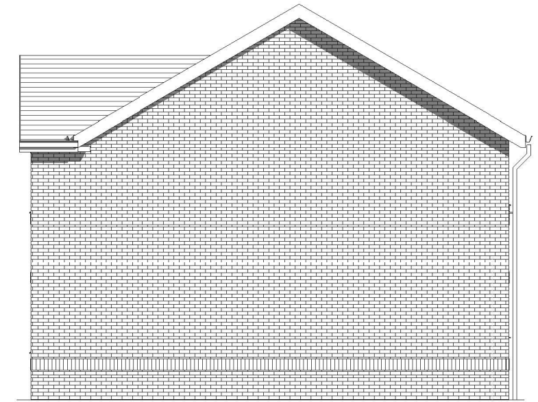
6 Existing Side 2 Elevation 1 : 100
