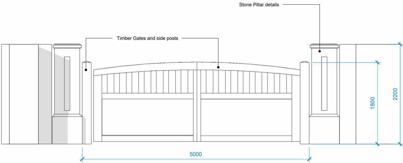
PROPOSED ENTRANCE GATE 1 : 50 ALL DIMENSIONS TO BE CHECKED ON SITE
