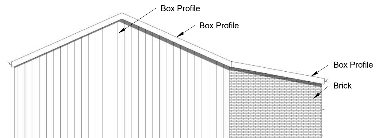
Existing & Proposed Side 2 Elevation
