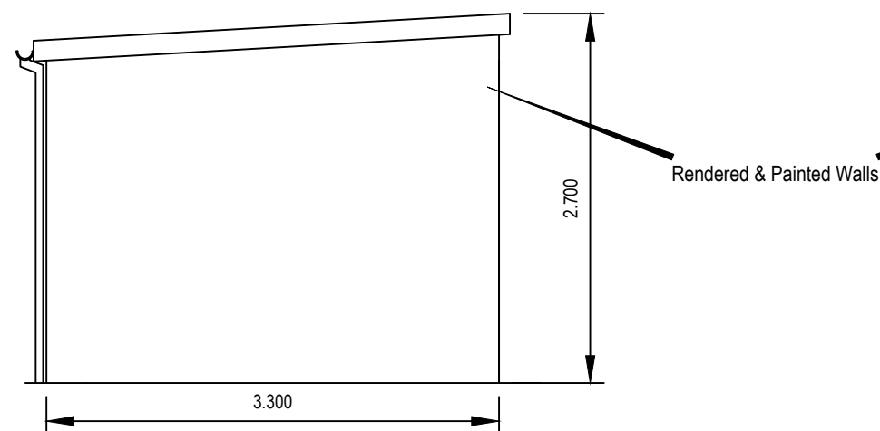
South Side Elevation
