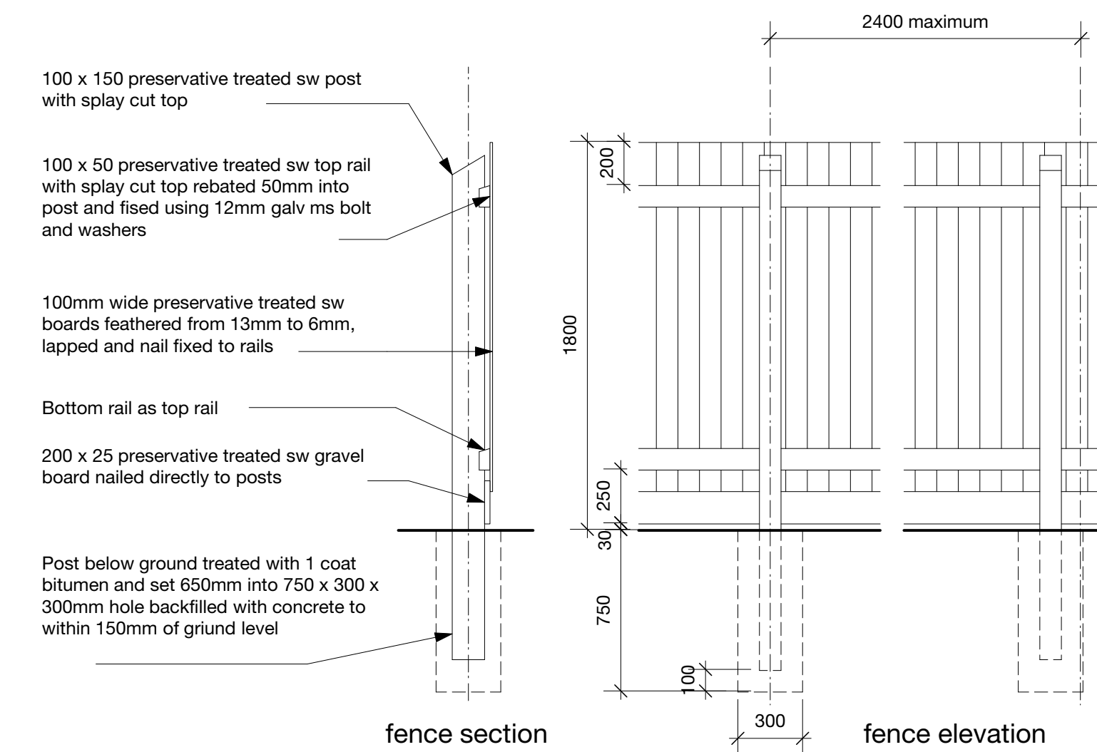
DETAILS OF FENCE G AND GATE H (1:25)
