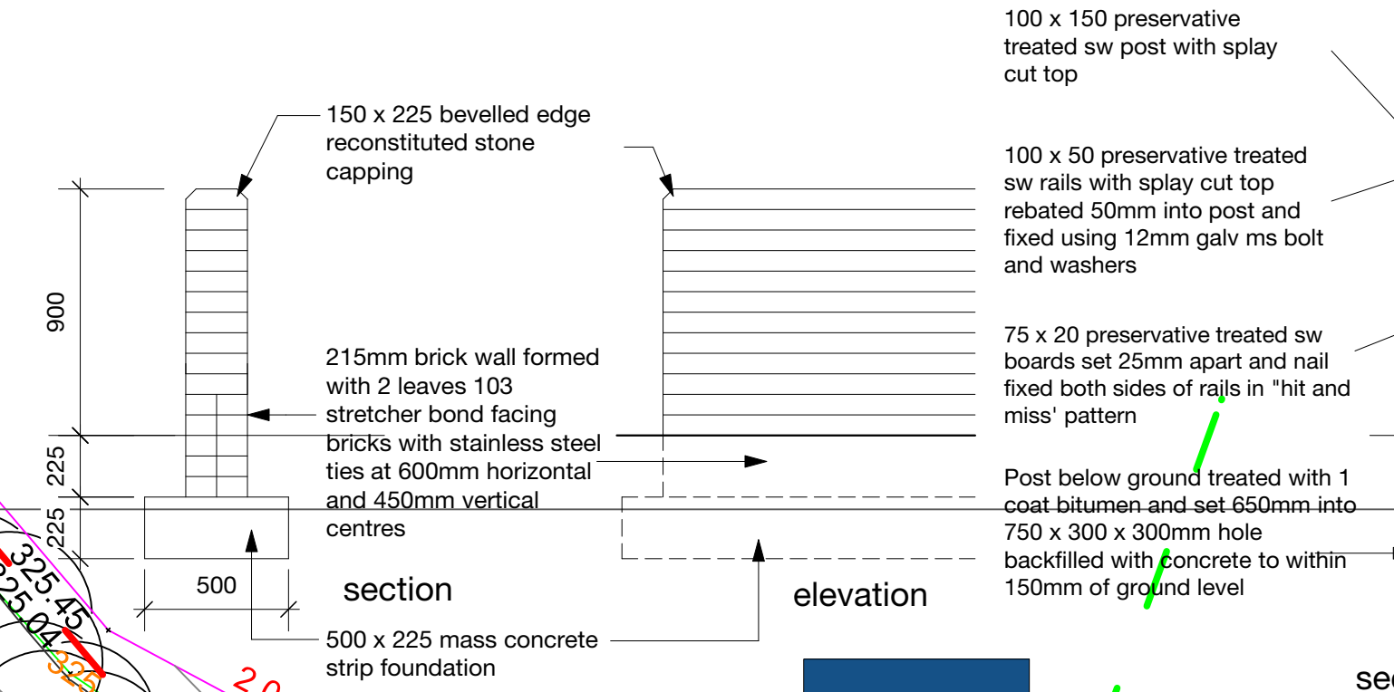
DETAILS OF FRONT GARDEN WALL(1:25)
