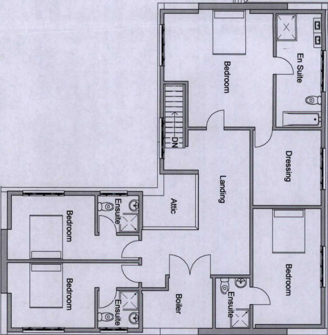
1 Proposed First Floor 1 : 100
