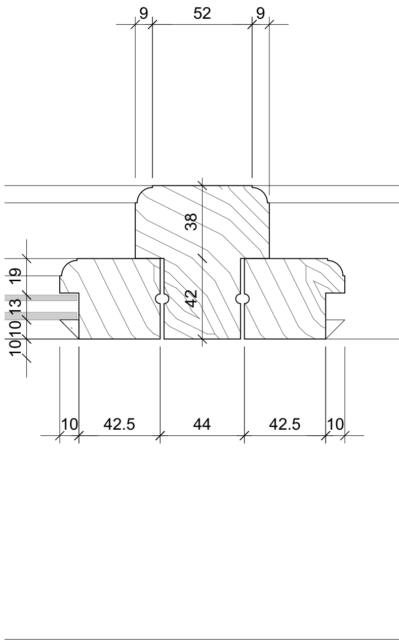
A 706.6 - MULLION SCALE 1:2
