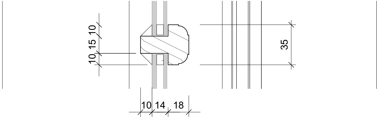
A 706.2 - GLAZING BAR SCALE 1:2
