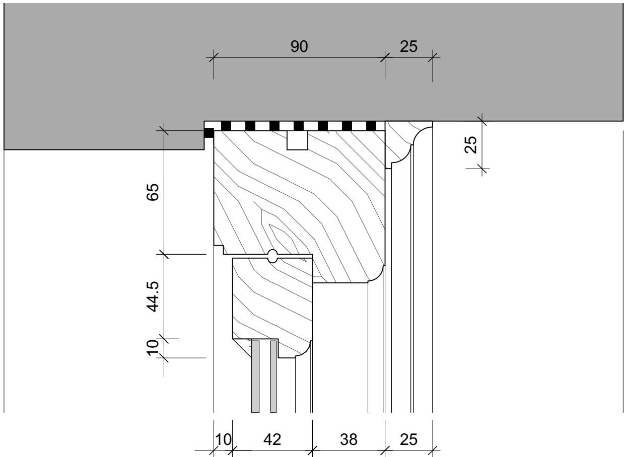
A 706.1 - HEAD SCALE 1:2
