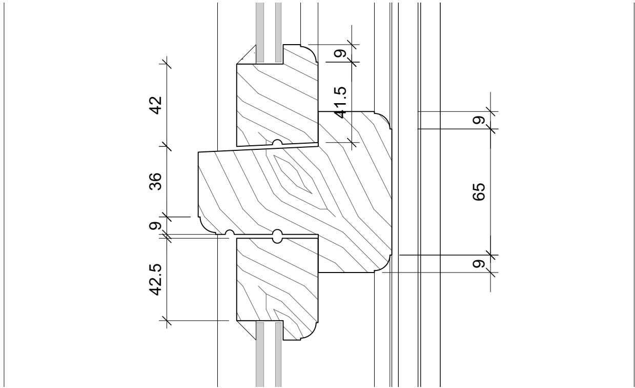
A 706.3 - TRANSOM BAR SCALE 1:2
