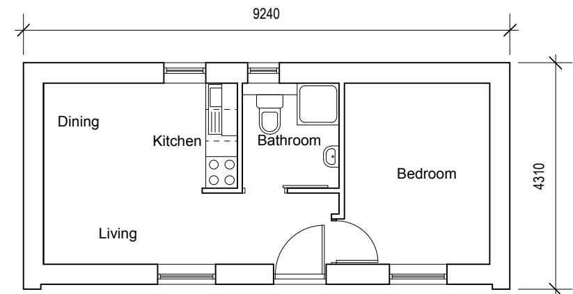
FLOOR PLAN
