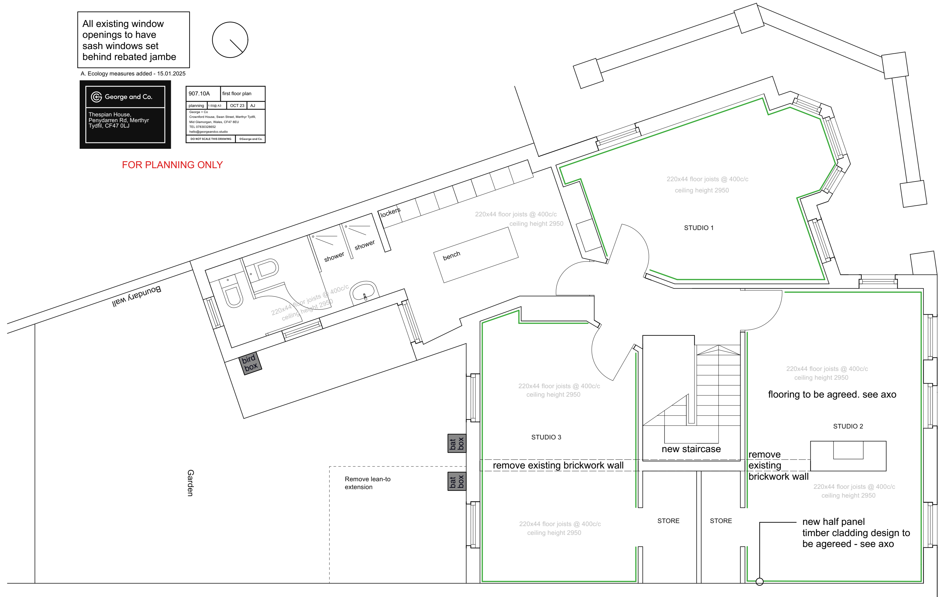
PROPOSED FIRST FLOOR
