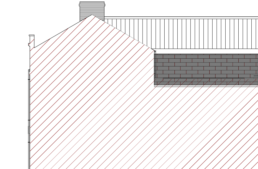
PROPOSED SIDE ELEVATION (EAST)
