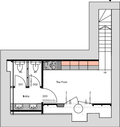
PROPOSED BASEMENT FLOOR LAYOUT
