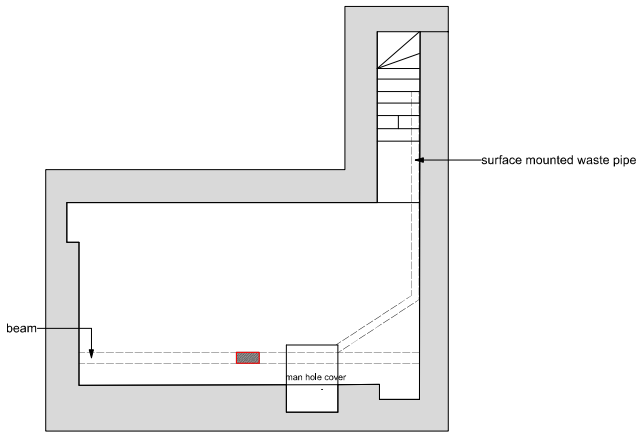
EXISTING BASEMENT FLOOR LAYOUT
