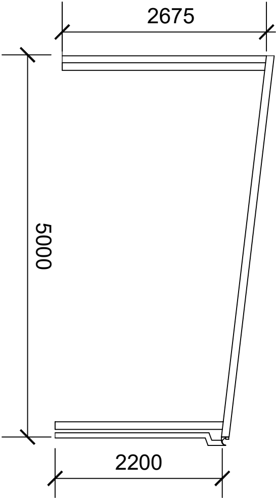
Side Elevation of Canopy
