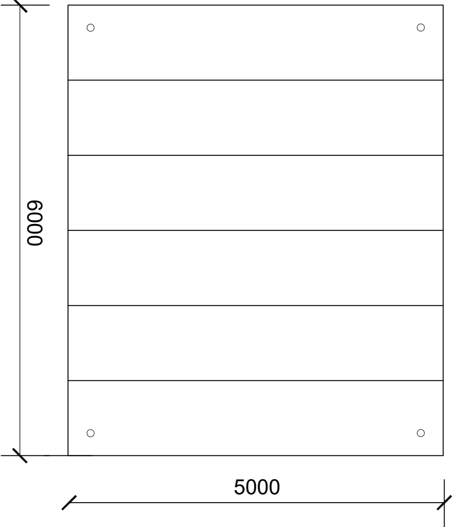
Plan of Proposed Canopy
