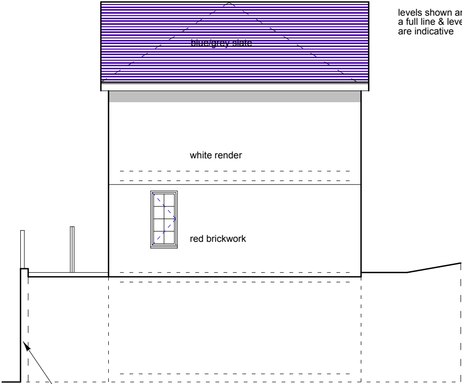
side elevation
