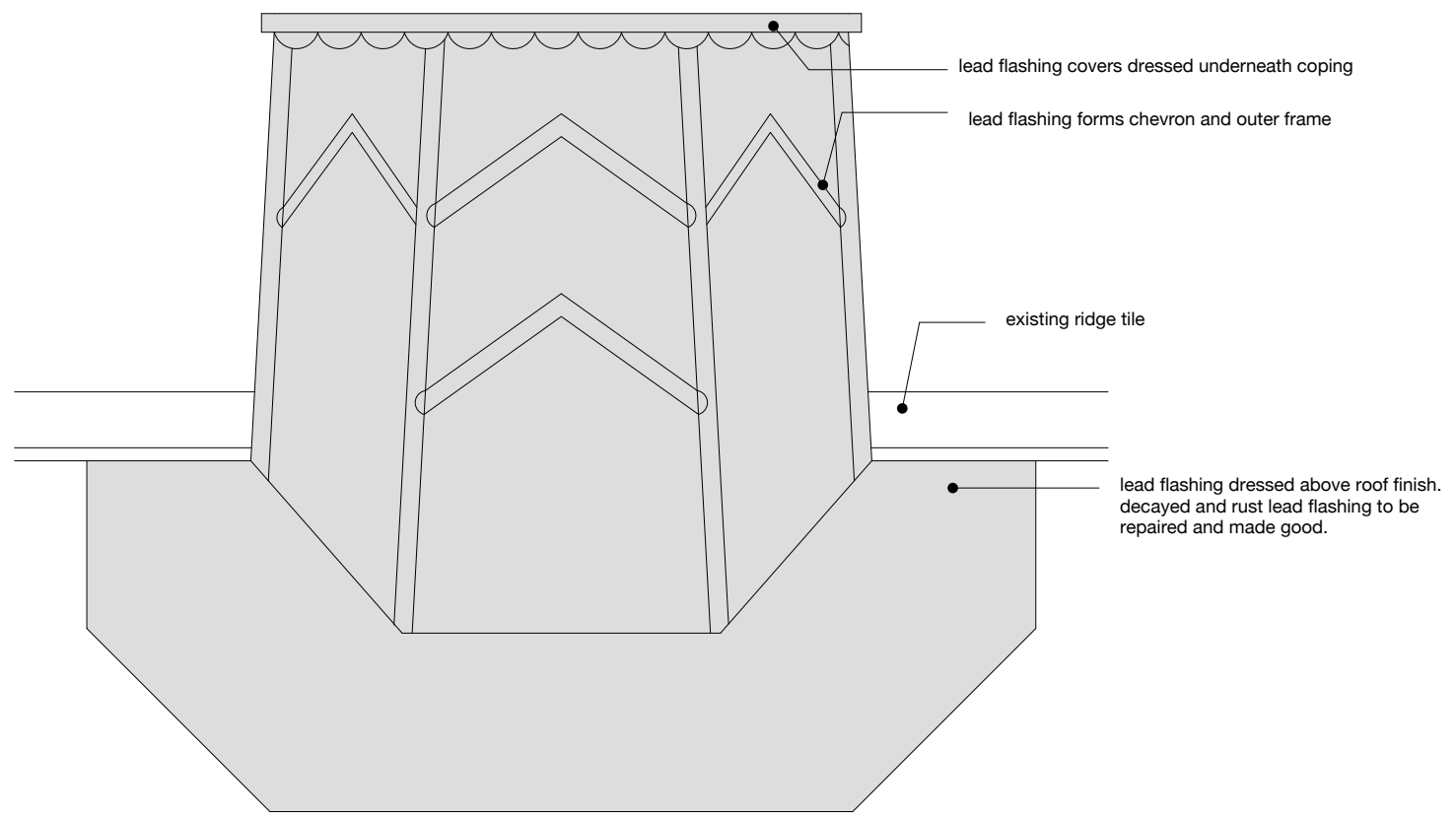
front and rear view
