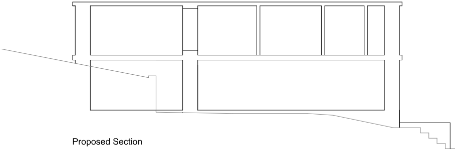
Proposed Section
