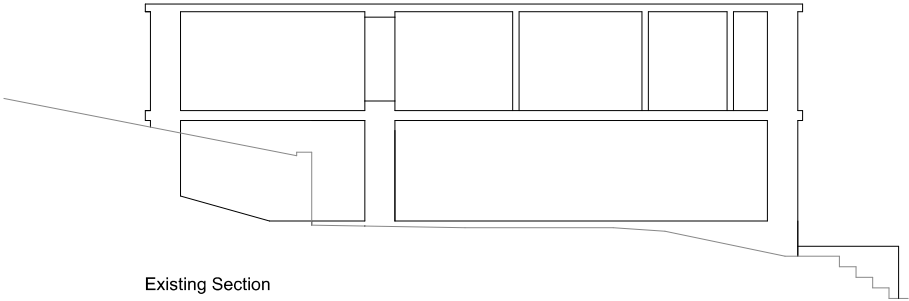
Existing Section
