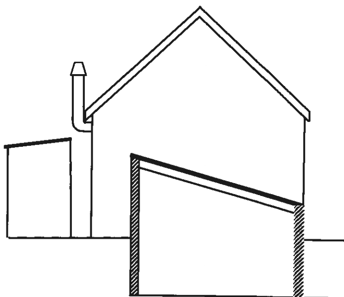
Proposed rear elevation with section through store
