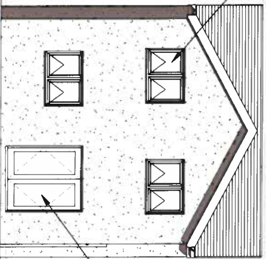
2 Proposed Rear Elevation 1 : 100
