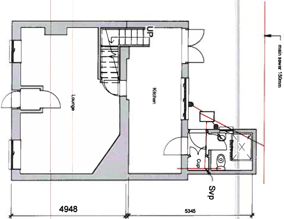
1 Existing Ground Floor 1 : 100 6701 front
